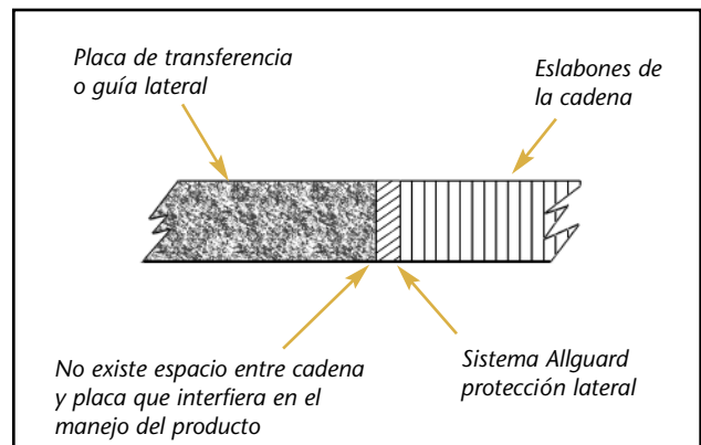
FIGURE 4 CADENA ALLGUARD
