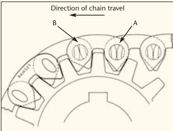
Ramsey Two Pin Joint
