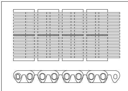
PASSO 1", GUIA CENTRAL
