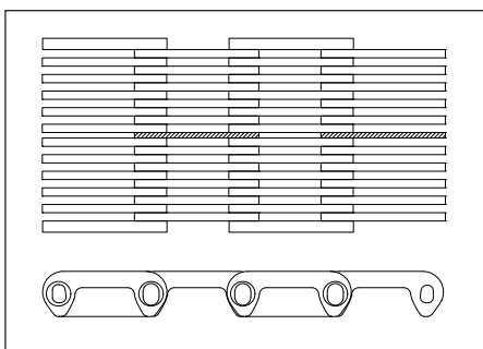
PASSO 1", GUIA CENTRAL
