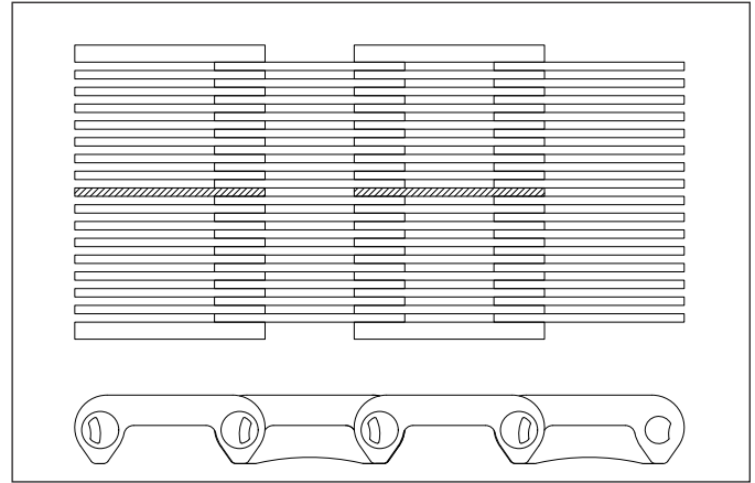
PASSO 1/2", GUIA LATERAL
