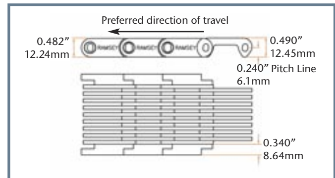
SINGLE PIN, 1 INCH PITCH
