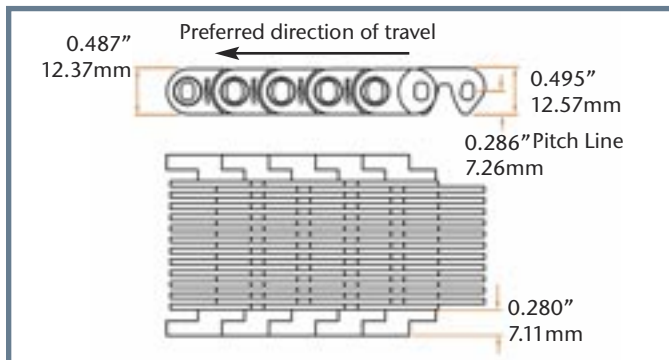
SINGLE PIN, 1/2 INCH PITCH
