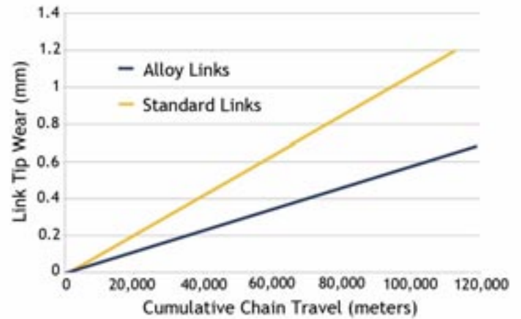
Improved Wear Resistance of Alloy Links
