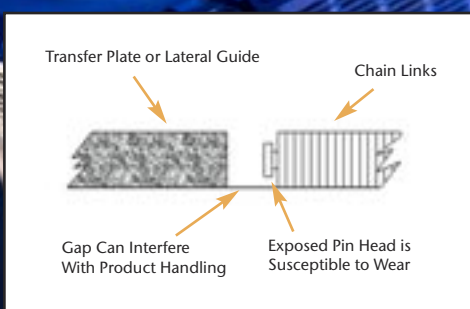
FIGURE 1 TYPICAL CONVEYOR CHAIN
